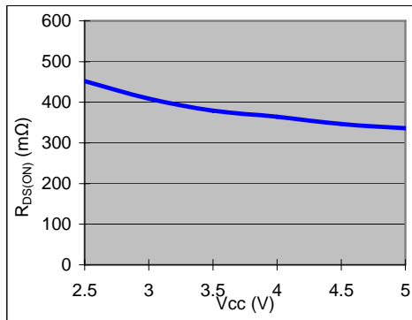
Vcc vs. R DS(ON)
